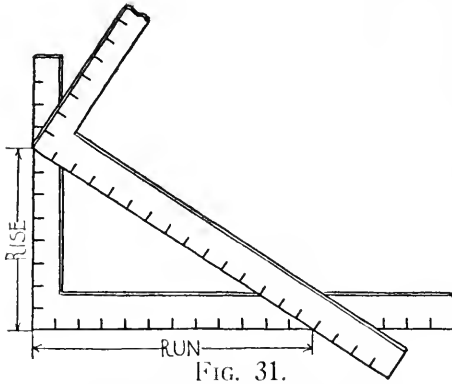
FIG. 31. OBTAINING RAFTER LENGTH BY SCALE METHOD.
